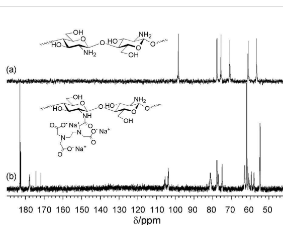
Fig. 2 13 C NMR spectra of (a) chitosan in DCI/D 2 O and (b) ED-ch 4a (D.S. 51%) in NaOD/D 2 O at rt.
