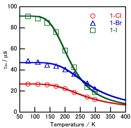
Figure 4. Temperature dependence of the average emission lifetimes of complexes 1-X in the crystals ( \lambda_{\text{ex}} = 337 \text{ nm} ). The solid lines were calculated by using eq. 2.
