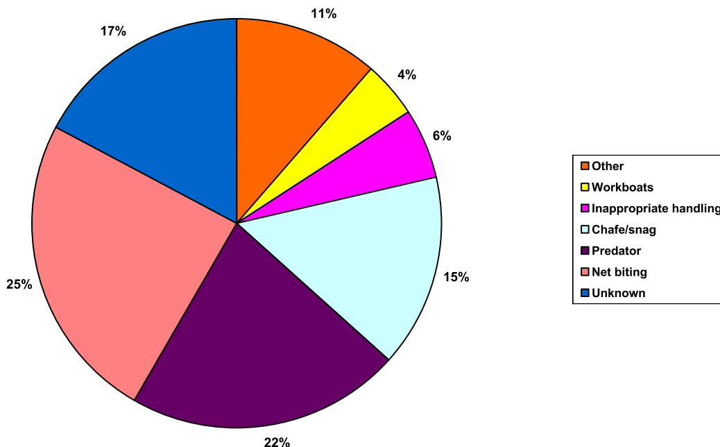
Fig. 3. Overall causes of hole in net. Number of incidents as a percentage of total incidences of hole in net.
