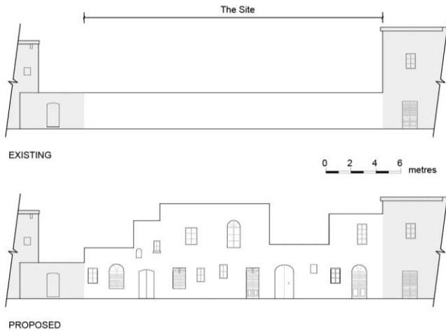
Figure 7. Existing and proposed elevation along the alley.
