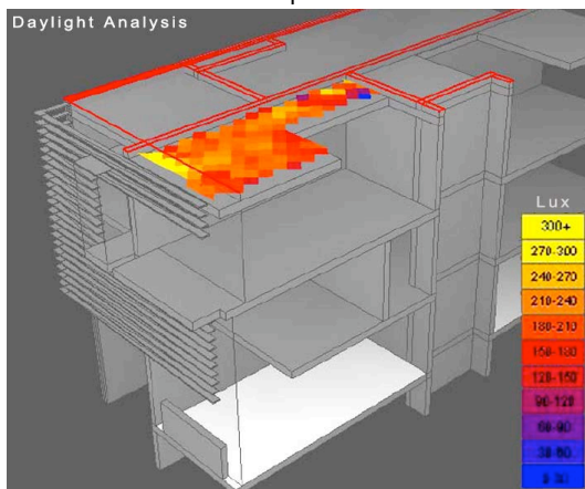
Fig 2. Lighting Analysis of louvered apartments
