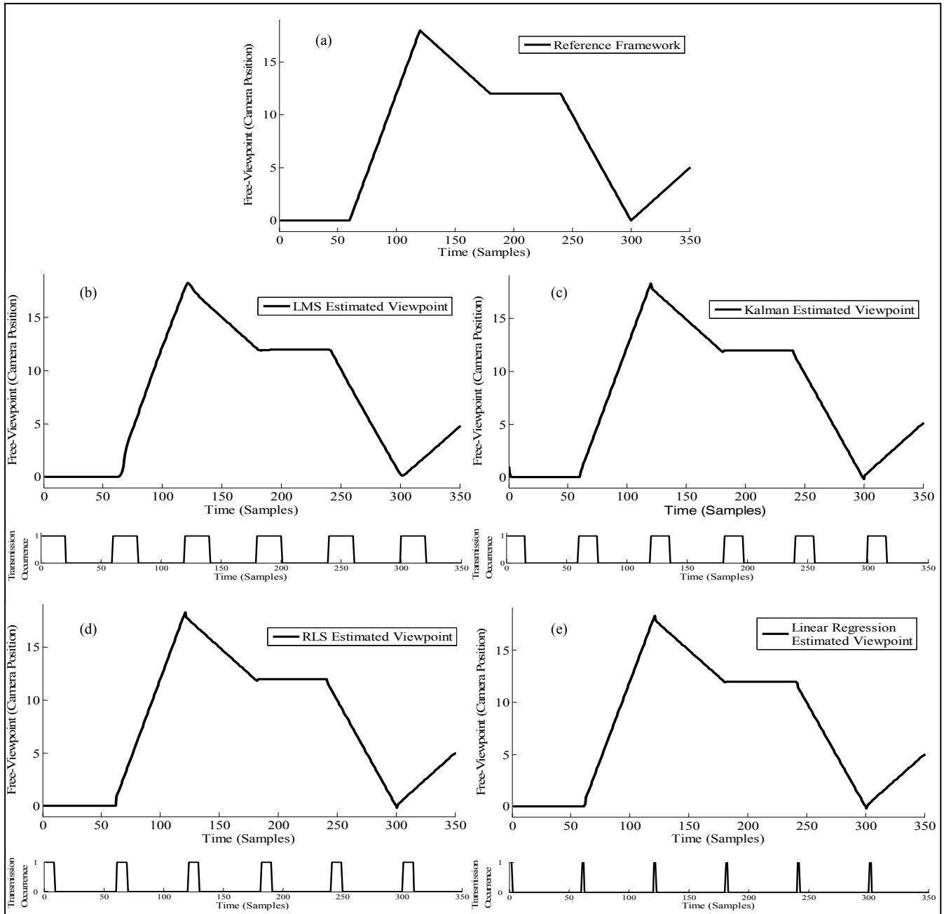
Figure 5. Simulation results and the associated transmission occurrences comparing the proposed algorithms in a typical FVV scenario for pattern A: (a) reference user input, (b) Least Mean Squares, (c) Kalman Filter, (d) Recursive Least Squares, (e) Linear Regression.
