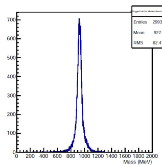
Figure 22. Missing mass reconstruction from two gammas where the particle identification is obtained by using the geometrical coincidence between the BGO calorimeter and the barrel scintillator[10].
