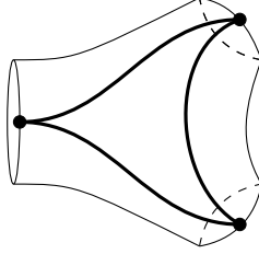
FIGURE 1. A natural embedding of \mathcal{A}(P) into S .
