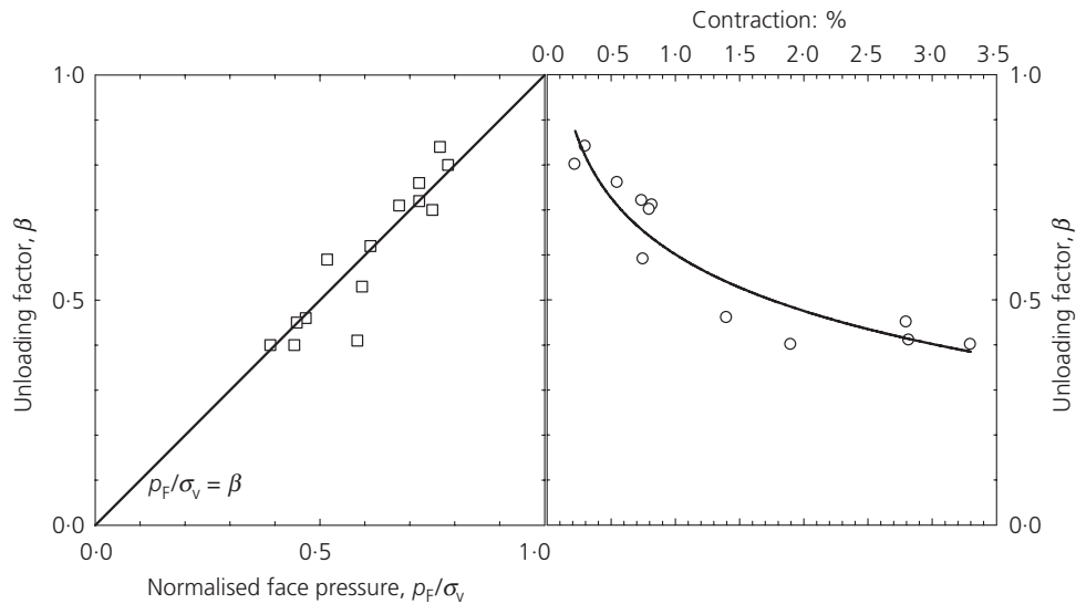
Figure 13. Relationships of contraction, stress reduction and modified grout pressure methods for all sections
