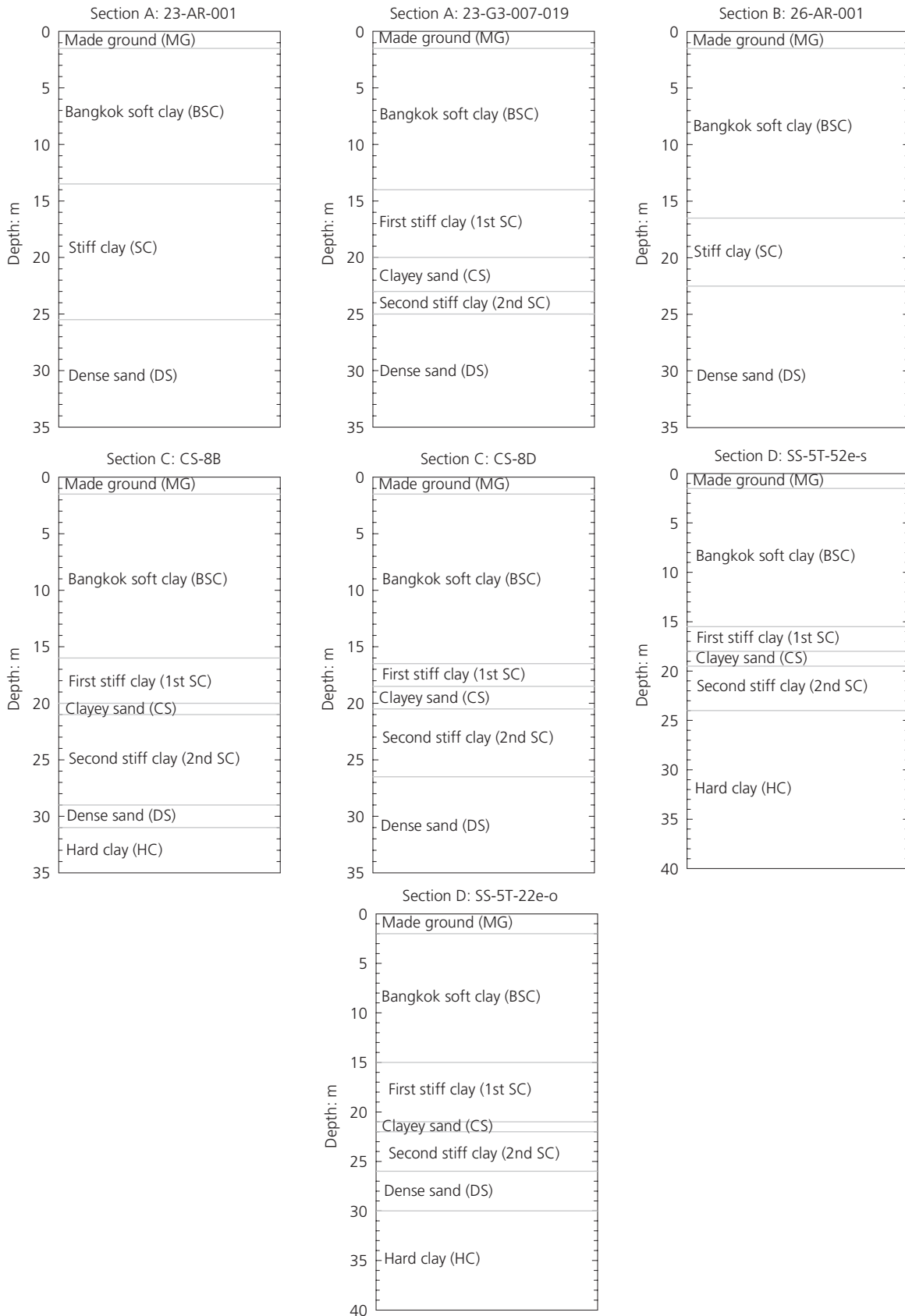
Figure 8. Soil profiles of seven sections analysed in the current study
