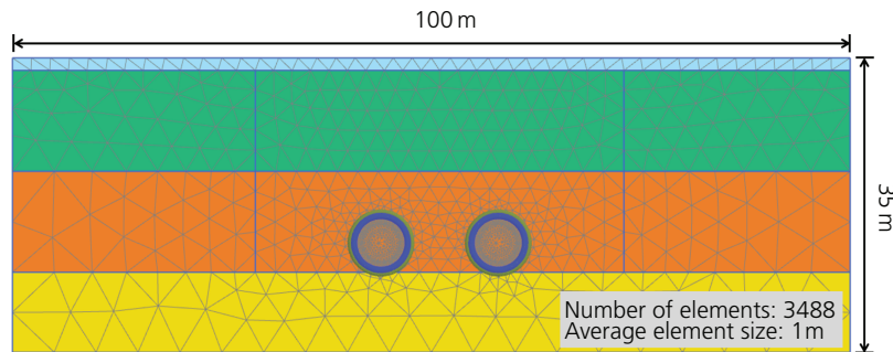
Figure 9. Typical finite-element model and mesh generation (an example from section A: 23-AR-001)
