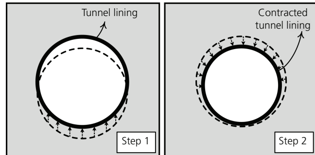
Figure 4. Calculation steps in contraction method
