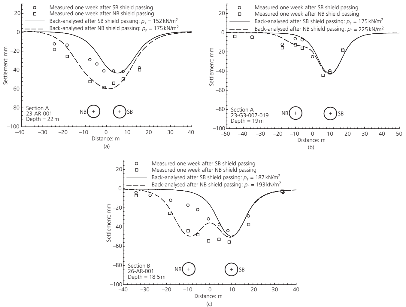
Figure 12. Results from modified grout pressure method: (a) section A: 23-AR-001; (b) section A: 23-G3-007-019; (c) section B: 26-AR-001; (d) section C: CS-8B; (e) section C: CS-8D; (f) section D: SS-5T-52e-s; (g) section D: SS-5T-22e-o (continued on next page)
