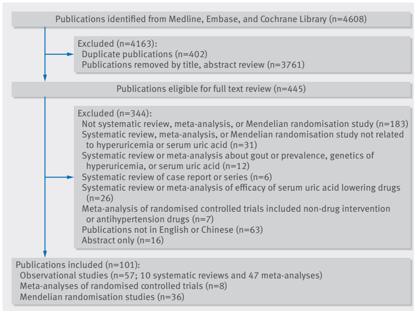
Fig 1 | Study flowchart
