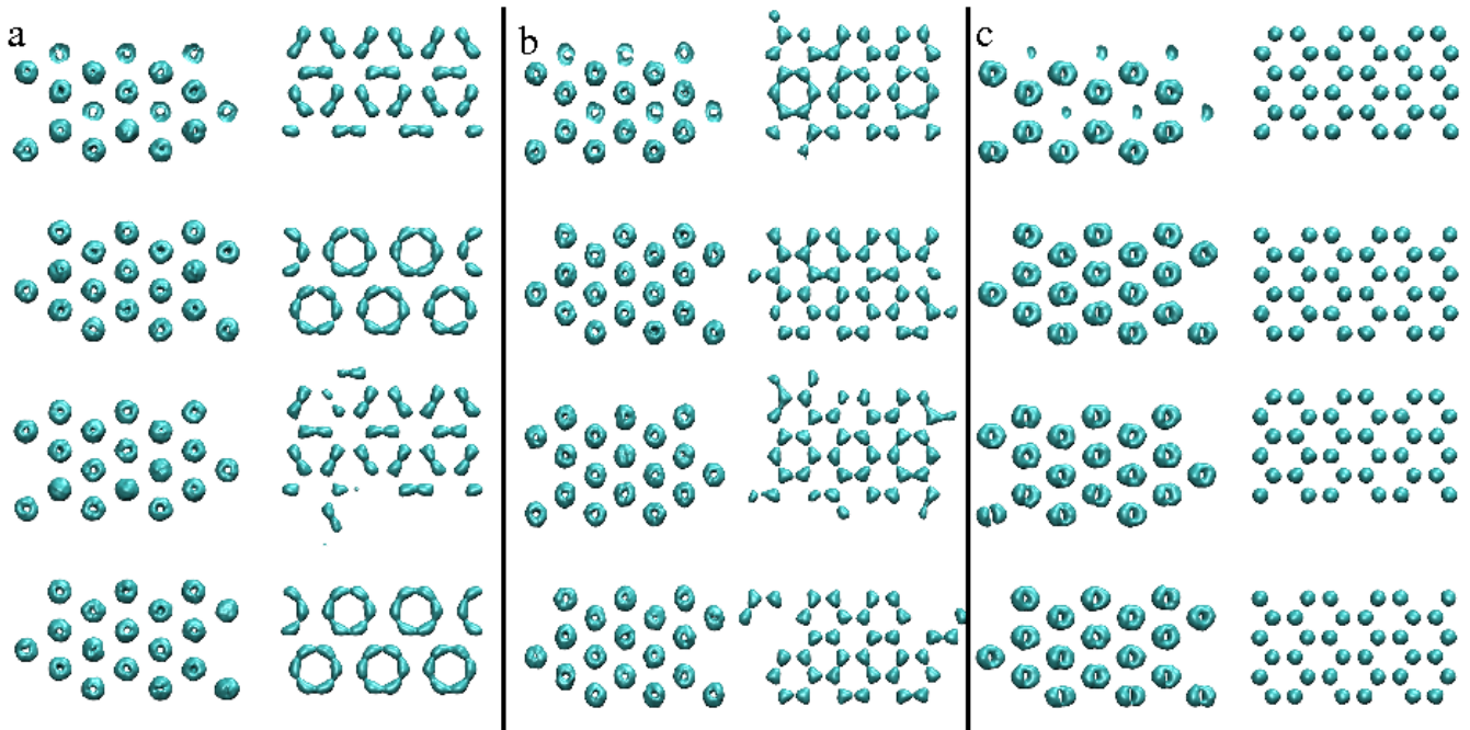
FIG. 2: Isosurfaces of time-averaged probability density for indistinguishable atoms from 8-layer AIMD simulations at different pressures. (a) 250GPa G'BG''B "Phase IV" (b) 325GPa BG' "Phase V" (c) 400GPa BG "atomic-molecular";
