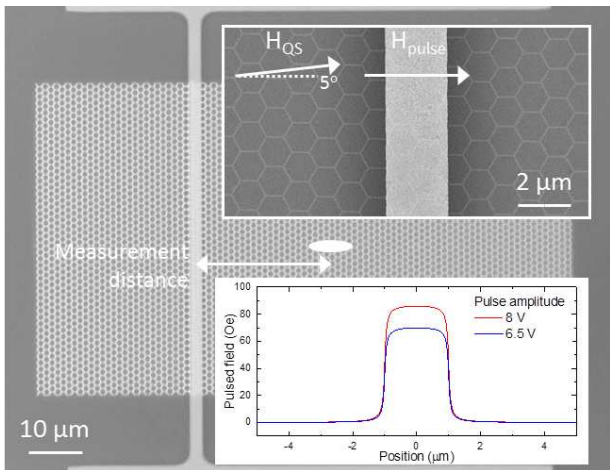
FIG. 2. Image of an interconnected array of nanowires with a Au stripline for applying localised pulsed magnetic fields. The geometry of the pulsed, H_{pulse} , and quasi-static, H_{QS} , fields is indicated with respect to the structuring. The ellipse indicates the position where measurements are made, a distance away from the stripline.
