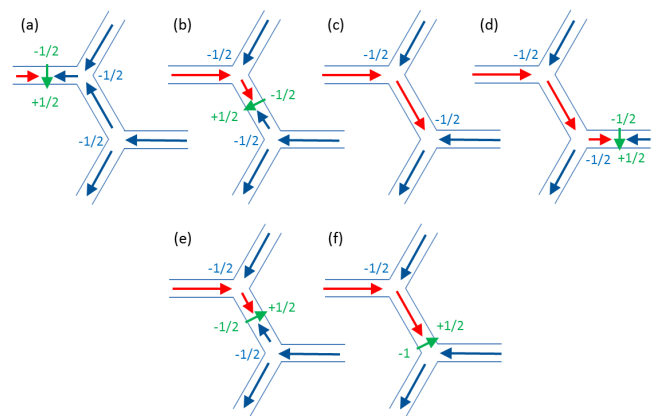
FIG. 1. Simple model of DW propagation and annihilation based on topological constraints in multiple vertices. The \pm 1/2 and -1 labels indicate the topological edge defects associated with the DW (green) and vertex (blue).
