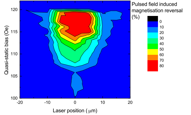
FIG. 5. Pulsed field induced magnetisation reversal measured as a function of quasi-static bias field and measurement position from the stripline. 20 ns Pulses at 7.5 V
