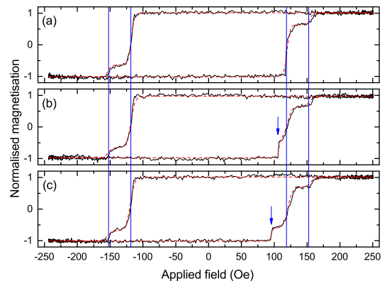
FIG. 3. MOKE hysteresis loops (black solid) showing the magnetisation reversal driven by (a) a quasi-static magnetic field and (b) and (c) with the addition of a pulsed magnetic field with triggering indicated by the arrows. The loops show the behaviour 9V 20ns pulses with the laser focused on top the stripline. The fitted lines (red dashed) show a model fit to the data.
