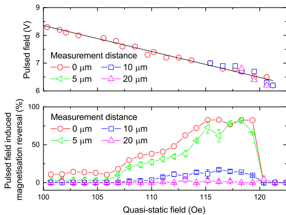
FIG. 4. a) Minimum pulsed voltage required to lead to magnetisation reversal when pulses are triggered at different quasi-static bias fields. b) Pulsed field induced magnetisation reversal as a function of quasi-static bias field measured at various distances from the DW injection stripline. Pulses are 20 ns and 7.5 V
