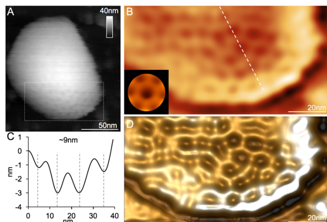
Fig. 3 Spatial organization of proteins in a partial \beta -carboxysome from the 30% fraction. (A) High-resolution AFM topograph of a partial \beta -carboxysome fragment in buffer. (B) High-pass-filtered AFM image showing the protein organization in the shell fragment depicted in (A). The white line of the cross section was used to calculate the pattern of hexamer organization in (C). (C) The cross-section profile illustrates the periodic arrangement of hexamers and the center-to-center distance between neighboring hexamers is \sim 9 nm. (D) Three-dimensional height image of the shell showing the shell protein structures and arrangement.
