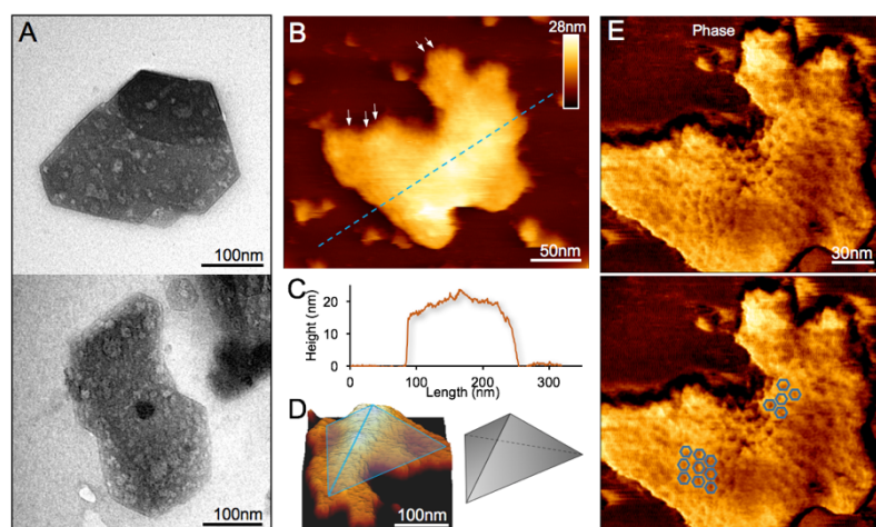
Fig. 2 Characterization of the \beta -carboxysome fragments in the 20% and 30% fractions. (A) TEM images of \beta -carboxysome fragments captured in the 20 and 30% fractions. Regular and straight facet edges and proteins associated with the facets were observed. More TEM images are shown in Fig. S2. (B) AFM topograph of a typical \beta -carboxysome fragment illustrating the spatial organization of individual shell proteins (indicated by arrows). AFM topograph of a curved \beta -carboxysome fragment is shown in Fig. 3. (C) Cross-section analysis of the \beta -carboxysome fragment along the dashed line indicated in (B). (D) 3D representation of the \beta -carboxysome fragment, showing the possible shell substructure comprises two shell facets that have a joint facet edge. (E) AFM phase image recorded together with the height image (B), displaying the native protein organization in the shell facets, with patterns of individual shell hexamers highlighted in blue hexagons.
