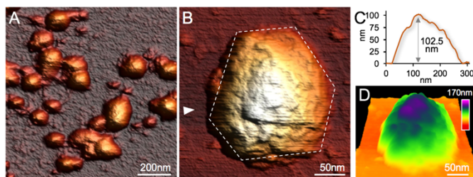
Fig. 5 Native AFM topographs of intact \beta -carboxysomes from Syn7942. (A) An overview topograph of isolated intact \beta -carboxysomes in the 40% fraction captured by AFM in solution. (B) High-resolution AFM image of a single intact \beta -carboxysome, showing the morphological features of \beta -carboxysomes. Several surface protrusions can be distinguished. The polyhedral shape of the \beta -carboxysome is outlined by white dashed lines. (C) Height profile of the \beta -carboxysome, taken along the white arrow indicated in (B). (D) 3D representation of the native architecture of the same \beta -carboxysome from Syn7942.
