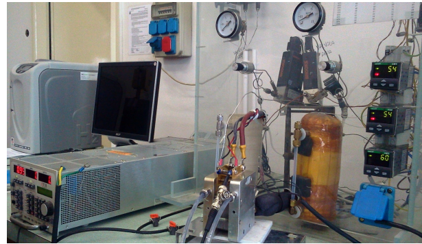
Fig. 6. Photograph of the experimental setup.
