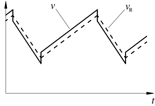
Fig. 5. Voltage response to the converter current ripple (solid line) according to the RL model (3) and its resistive component (dashed line).
