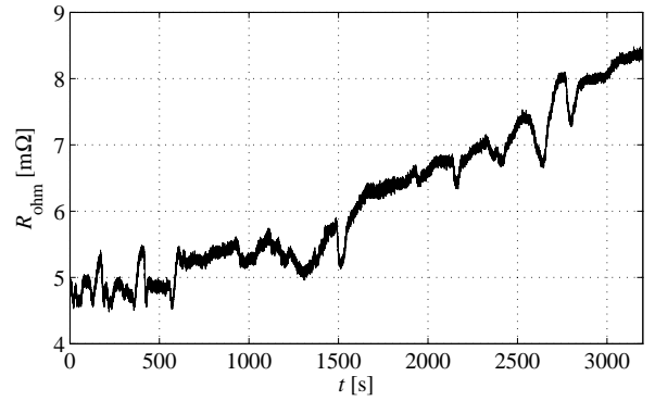
Fig. 10. Real-time ohmic resistance estimate calculated by the Compact-RIO during a membrane dehydration transient induced by decreasing the inlet gas relative humidity.
