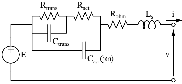
Fig. 3. Typical linearized equivalent circuit of a PEM FC.
