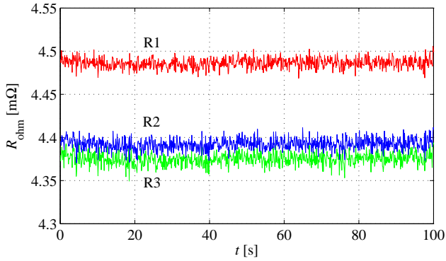
Fig. 9. Ohmic resistance values estimated off-line by different identification methods, namely the proposed time-domain analysis with (red line R1) and without (green line R3) elimination of extreme ramp values, and frequency-domain analysis (blue line R2).
