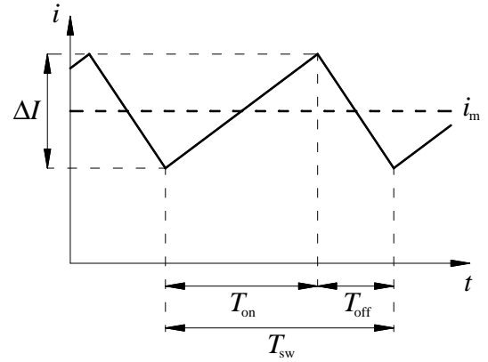
Fig. 2. Theoretical current waveform produced by the DC/DC converter.
