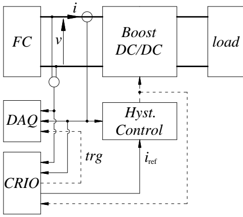
Fig. 7. Schematic drawing of the connections among the employed devices.
