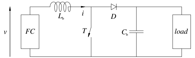
Fig. 1. Schematic representation of a DC/DC boost converter connected to the FC on one side and to an electrical load on the other side.
