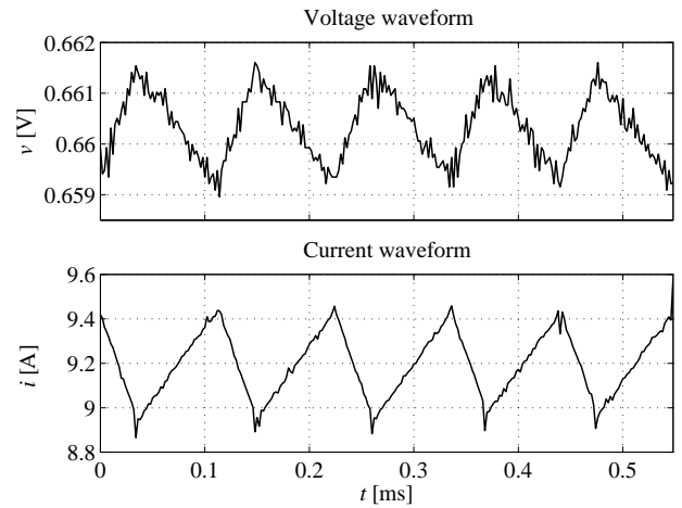
Fig. 8. Current and voltage waveforms measured by the DAQ system.
