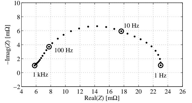
Fig. 4. Impedance spectrum of the cell under test, measured at 9.2 A DC current in typical operating conditions.
