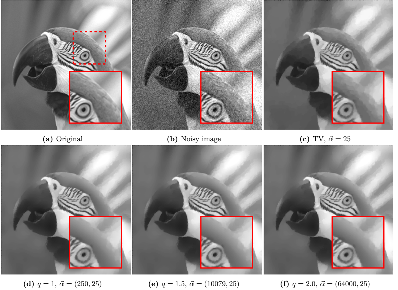
Figure 1: Effect of the of exponent q in the norm \|\mathcal{E}w\|_{F, L^q(\Omega; \text{Sym}^2(\mathbb{R}^m))} in variants of TGV 2 together with fidelity \phi(t) = t^2/2 . The \beta factor has been scaled from the case q = 1 with the help of the Cauchy-Schwarz inequality. There is no discernible difference between the results for different q , all having PSNR 29.2, while the TV comparison has PSNR 28.0 and exhibits the stair-casing effect in the sky that TGV 2 variants do not.
