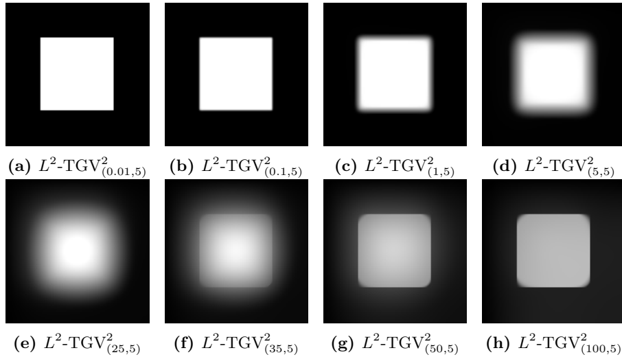
Figure 5: Illustration for \alpha = 5 of varying \beta parameter for \text{TGV}^2 regularisation with squared L^2 fidelity on f = \chi_{(-32,32)^2} .
