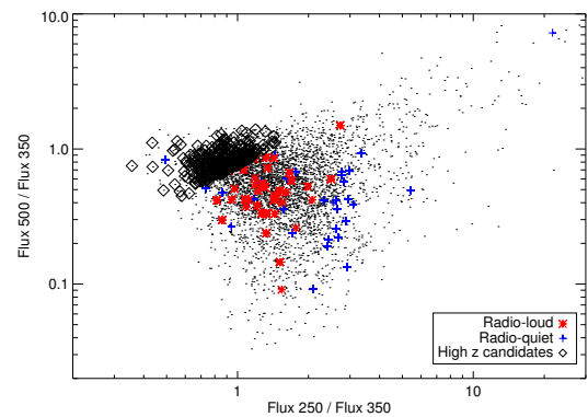
Figure 4. Colour-colour plot of 250\mu\text{m}/350\mu\text{m} ratio against 500\mu\text{m}/350\mu\text{m} ratio. Red and blue dots indicate radio-loud and radio-quiet objects respectively. Possible high redshift galaxies are shown as bold points, which cluster in the area of higher 500\mu\text{m}/350\mu\text{m} ( > 0.4 ) and lower 250\mu\text{m}/350\mu\text{m} ( < 1.5 ) ratios.
