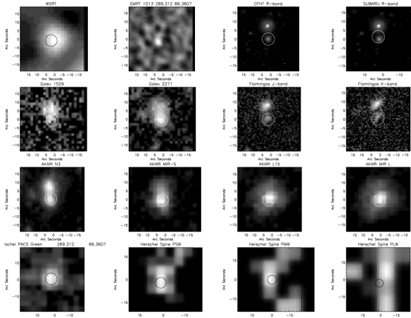
Figure 2. 40'' \times 40'' images centred on the WSRT radio source NEP 175714+662139. The circle is a nominal 4'' diameter reference at the position of the WSRT radio source, to show the relative positional accuracy of the various surveys.
