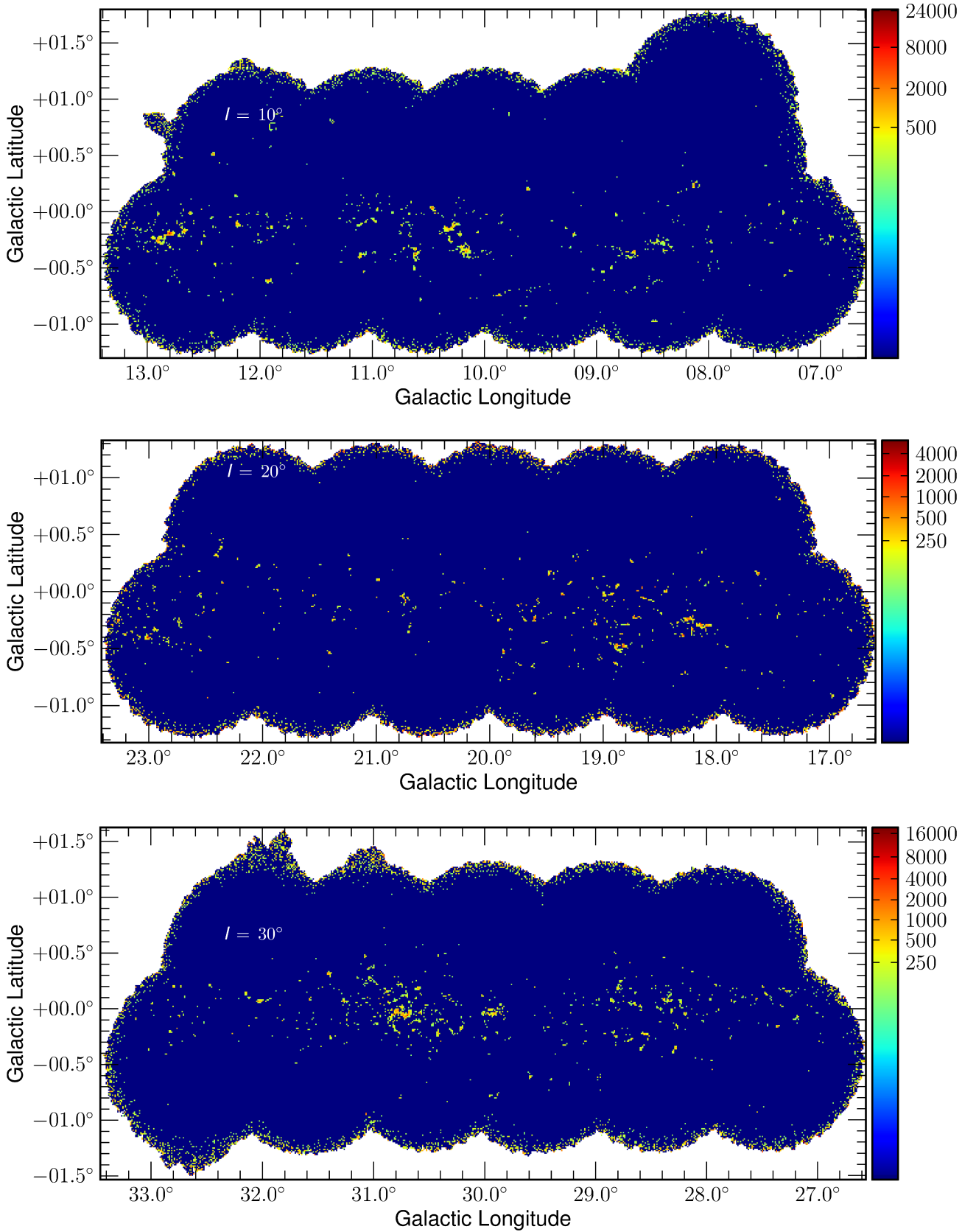
Figure 1. The JPSPR1 maps for the first three fields, l = 10^\circ , 20^\circ and 30^\circ . The intensity scale is in units of \text{mJy beam}^{-1} . Several areas can be seen where the SCUBA-2 instrument continued to take data beyond the edge of the standard circular pong3600 tile. These excursions are visible at the edges of most of the fields and the l = 10^\circ field is misshapen in the top right tile. This extension is caused by the inclusion of a trial observation taken prior to the main survey that has a small positional offset from the standard grid pattern. Significant regions can be observed in each field with W31 found at l = 18.25^\circ , b = -0.19^\circ , W39 at l = 18.86^\circ , b = -0.48^\circ and G29 and W43 found at l = 29.95^\circ , b = -0.02^\circ and l = 30.75^\circ , b = -0.05^\circ , respectively.
