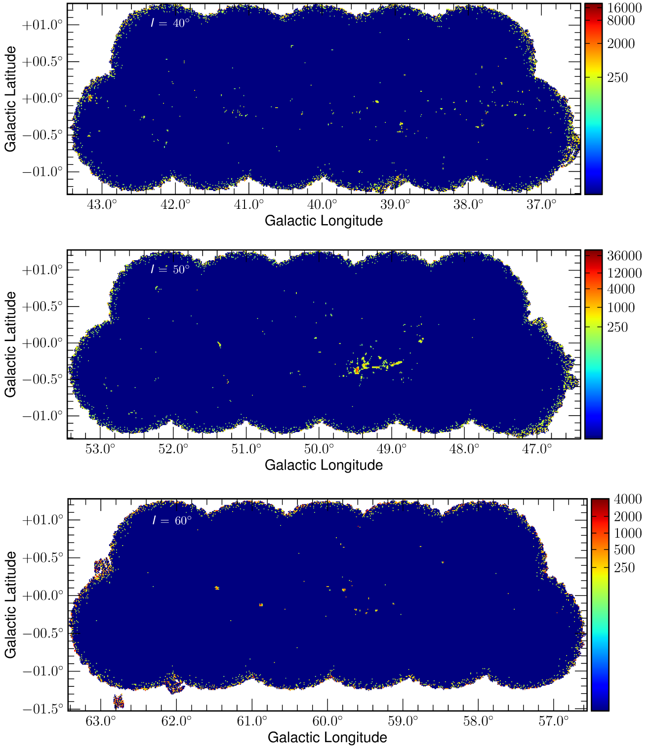
Figure 2. The JPSPR1 maps for the three fields centred at l = 40^\circ , 50^\circ and 60^\circ . The intensity scale is in units of \text{mJy beam}^{-1} . The W51 star-forming region can be located at l = 49.40^\circ , b = -0.38^\circ .
