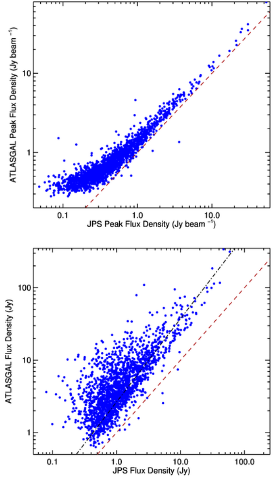
Figure 3. Comparison of the JPS sources with the spatially corresponding ATLASGAL clumps. Top panel: peak flux densities. Bottom panel: integrated flux densities. The red dashed lines correspond to the 1:1 line, with the black dot-dash line representing the linear fit to the matched integrated flux densities.
