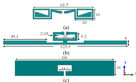
Fig. 1. Tag antennas with dimensions in mm (a) Tag 1 (b) Tag 2 (c) Tag 3.
