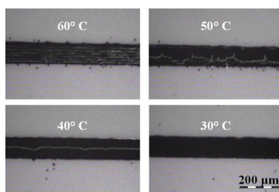
Fig. 2. Effect of platen temperature on printed pattern.
