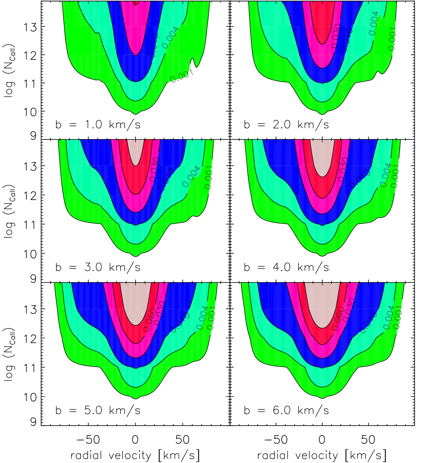
Fig. 9. Difference between S_{E=100} and S_{\text{MW}} obtained by varying the ISM broadening ( b -parameter), radial velocity (RV), and column density ( \log N_{\text{CaII}} ), keeping E fixed at 100 \text{ erg cm}^{-2} \text{ s}^{-1} . The values along the lines of each contour (0.001, 0.004, 0.01, 0.03, 0.06, 0.11) quantify the S_{E=100} - S_{\text{MW}} difference.
