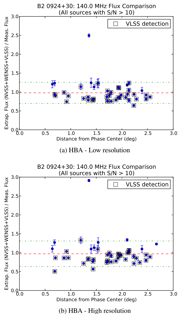
Fig. 1: Ratio of measured and catalogue extrapolated flux densities for our high- and low-resolution averaged LOFAR images.
