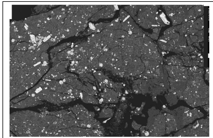
Fig. 1. BSE Image of Carancas clast. View measures 0.5 mm across. Magnetite and sulfides are white, most of the remainder is phyllosilicates and carbonates.
