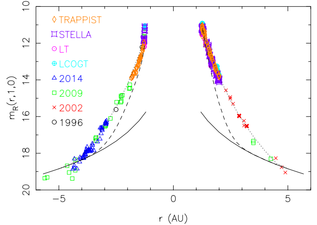
Figure 3. Total R -band magnitude within \rho = 10,000 km, corrected to unit geocentric distance and zero degrees phase angle, against heliocentric distance. The solid line shows the predicted magnitude of the inactive nucleus, the dashed line a prediction based on the expected total water prediction rate, and the dotted line an empirical prediction based on photometry from previous orbits (see Snodgrass et al. 2013, for details)
