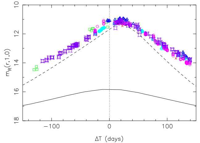
Figure 4. Same as Fig. 3, but plotted against time from perihelion (days) and showing only the near-perihelion period ( \pm 150 days).
