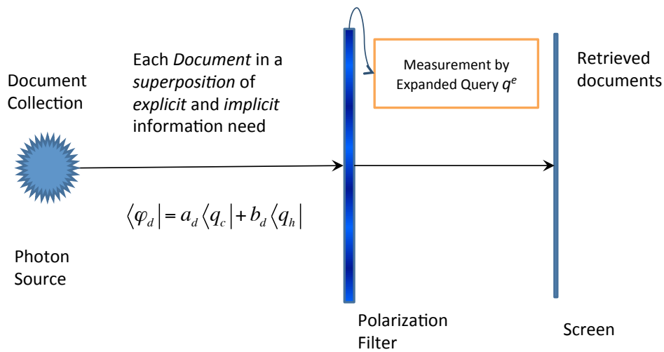
Figure 5. Unknown path (be \varphi_d \mapsto q_c \mapsto q^e and \varphi_d \mapsto q_h \mapsto q^e simultaneously) for documents as photons that pass the measurement filter. In such uncertain cases entailed by the superposition state, the quantum interference can possibly occur.
