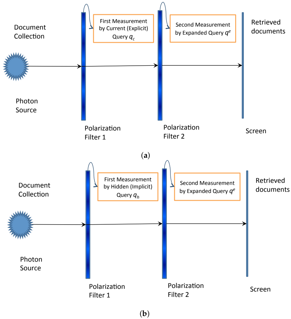
Figure 4. (a) First measurement by current query |q_c\rangle , (b) First measurement by hidden query |q_h\rangle . Known Paths \varphi_d \mapsto q_c \mapsto q^e (in subfigure (a)) and \varphi_d \mapsto q_h \mapsto q^e (in subfigure (b)) for documents as photons that pass the measurement filters. In each certain condition, the quantum interference can not occur.
