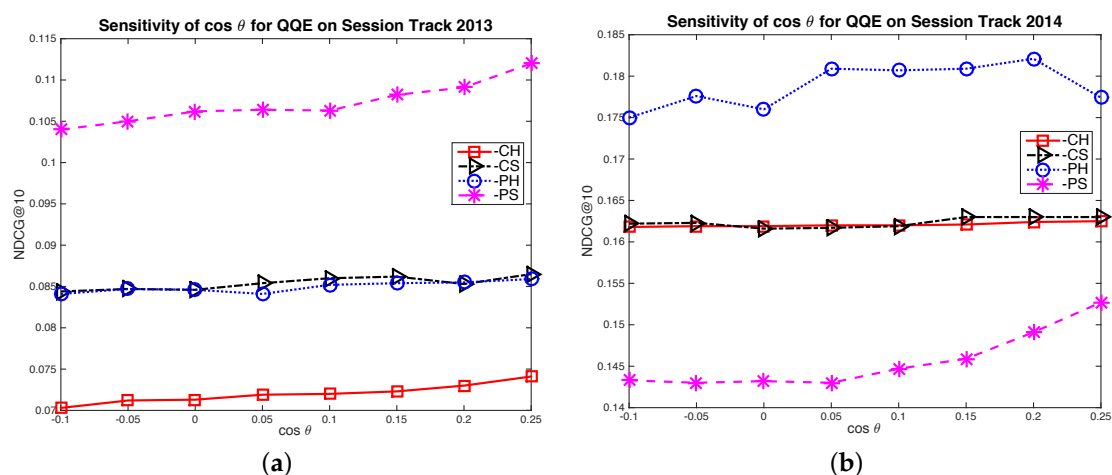
Figure 6. The effect of quantum interference term by observing the sensitivity of \cos \theta on (a) TREC 2013 and (b) TREC 2014.
