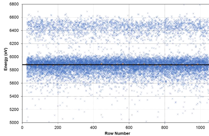
Figure 3: X-ray scatter plot measured at 188 K using node F of device #10092-04-03, the peak locations and resulting linear fit used to calculate the parallel CTI are also included
