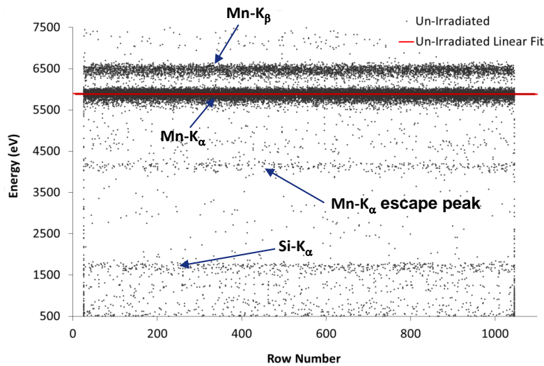
Figure 4: X-ray scatter plot measured at 153 K using node F of device #10092-04-05 pre-irradiation, the resulting linear fit used to calculate the parallel CTI is also included
