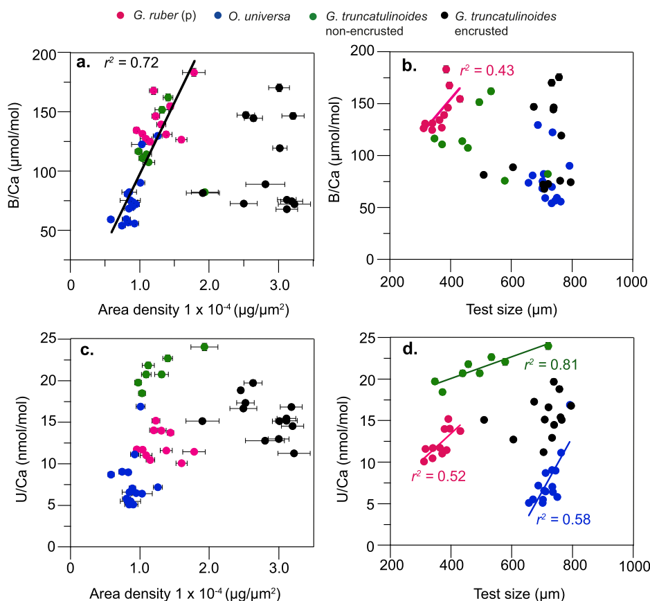
Fig. 4. Linear regressions of a ) B/Ca and area density of G. ruber (p), O. universa , G. truncatulinoides non-encrusted. Encrusted G. truncatulinoides are shown in black but are not included in the regression. b ) B/Ca with test size for all species. The only significant regression is in G. ruber (p) c ) U/Ca and area density for all species with only G. truncatulinoides non-encrusted/encrusted included in the regression. d ) Individual species' shell size regressions with U/Ca of G. ruber (p), O. universa , G. truncatulinoides non-encrusted/encrusted. Errors on area density measurements are AD \pm (1/n) , and B/Ca = \pm 1.84\% , U/Ca = 1.79\% (\pm \sigma) .
