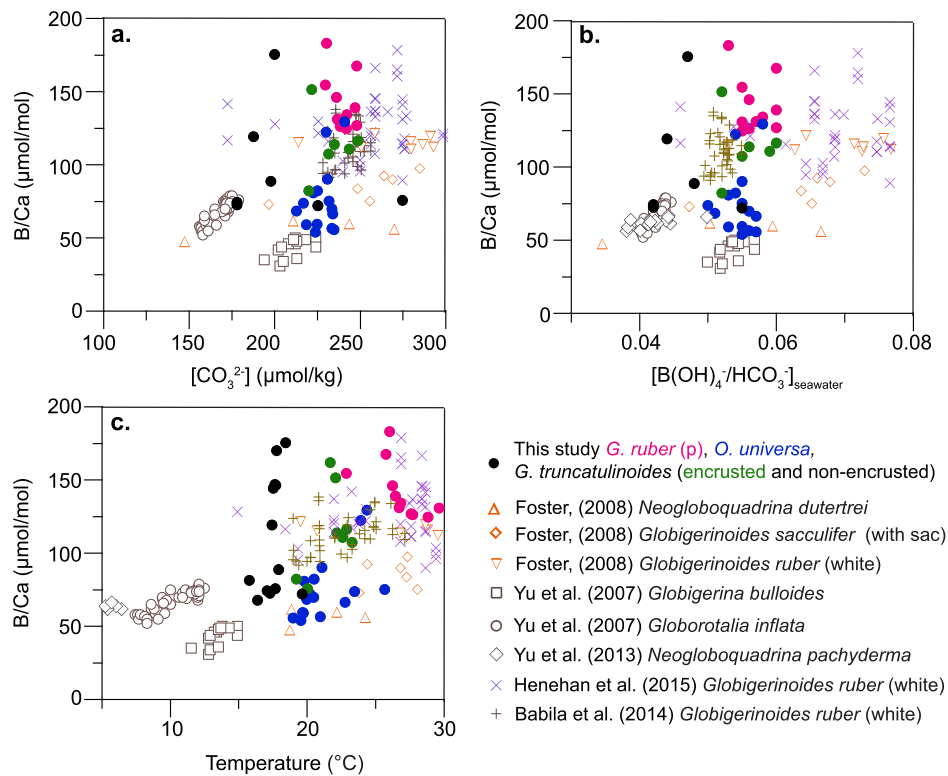
Fig. 3. Potential controls on boron incorporation: B/Ca from this study and other planktonic species varying with a) [CO 3 2- ] and b) [B(OH) 4 - ]/[HCO 3 - ] seawater c) Temperature. Data from Babila et al. (2014) is an average of 20–40 m. Figures show open-ocean data only.
