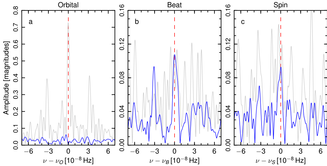
Extended Data Figure 6: Amplitude spectra from 7 years of sparsely-sampled CSS data. a-c , The amplitude as a function of frequency relative to the mean orbital ( a ), beat ( b ) and spin ( c ) frequencies listed in Extended Data Table 2. The grey line is the spectrum without any processing; the blue line is the spectrum after subtraction of the orbital signal.
