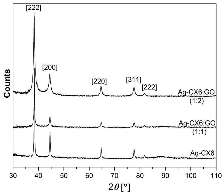
Figure 2. XRD patterns for Ag and Ag-Graphene nanocomposites
