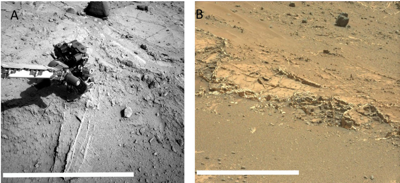
Fig. 1. A) Sulfate veins prominent at Darwin outcrop veins, observed on sol 402, NavCam NRB_432923862. Field of view 1.3 m. B) Garden City image, observed on sol 924, MastCam ML004061. White sulfate veins cut through the surrounding sediments. Scale bars are 1 m.
