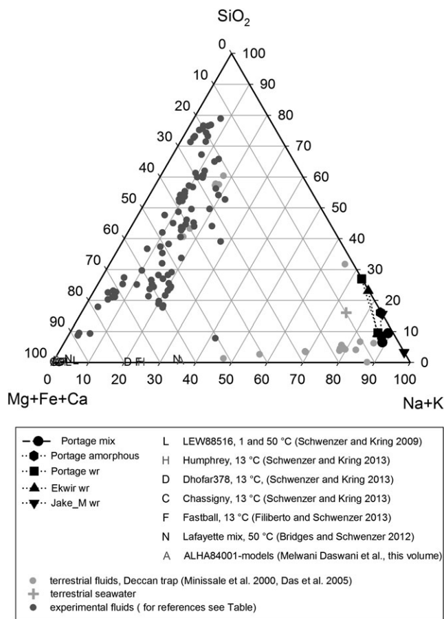
Fig. 6. Ternary plot showing the relationship between the dissolved alkaline earth metals (plus Fe), and dissolved silica. We include Fe with the alkaline Earth elements because it frequently occupies the same crystallographic sites in host rock and alteration minerals. We note, however, that Fe concentrations are generally low in solution because of its low solubility in the presence of oxygen. In most modeling and experimental fluids, the partial pressure of oxygen is high enough for Fe-oxides or hydroxides to form. For references of the experimental fluids, see Table 2. Note that some of the Deccan Trap fluids fall into the alkali-rich corner of the plot, while others are particularly alkali-poor compared to their relative content in alkaline earths and silica.
