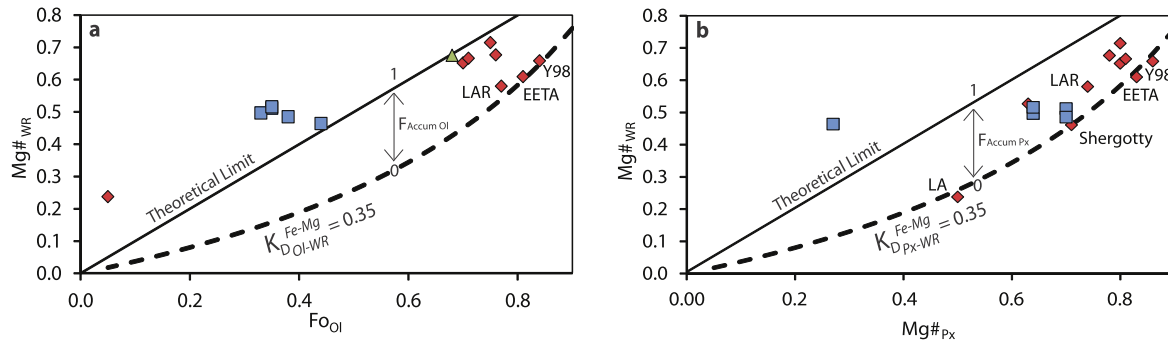
Fig. 2. The amount of a) olivine and b) pyroxene accumulation calculated for whole-rock compositions, assuming a K_{D}^{\text{Fe-Mg}} = 0.35 . Samples plotting on the dashed lines resemble liquid compositions, where increasing vertical departure from the equilibrium curve is proportional to the fraction of the accumulated mineral, where the theoretical limit is \text{Mg\#}_{\text{WR}} = \text{Mg\#}_{\text{Min}} .
