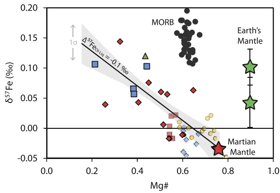
Fig. 6. Iron isotope compositions of SNCs corrected for olivine/pyroxene accumulation assuming a \Delta^{57}\text{Fe}_{\text{Min-Melt}} = -0.1\text{‰} (black line). The Martian array, including associated 1\sigma uncertainty (grey envelope) is lighter than MORB (black circles) and the Earth's primitive mantle (green stars) at a given Mg#, leading to a mantle composition (red star) within uncertainty of chondrites. Chondrites: Enstatite = red squares, Carbonaceous = blue diamonds, Ordinary = yellow circles; iron isotope data from Needham et al. (2009); Poitrasson et al. (2004); Schoenberg and von Blanckenburg (2006), and Craddock and Dauphas (2011). MgO values from Jarosewich (1990). (For interpretation of the references to colour in this figure legend, the reader is referred to the web version of this article.)
