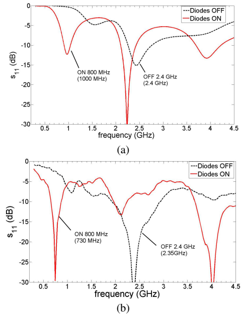
Fig. 2 Plots of S_{11} parameter for the (a) simulated and (b) measured antennas, for the diodes ON and OFF. With the diodes OFF, operation is at 2.4 GHz and ON at 800 MHz (larger effective structure size).
