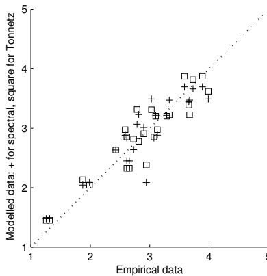
Figure 5. A scatter plot showing the relationship between the empirical data ( x -axis) and their modelled values ( y -axis). The spectral pitch-class model is indicated with the + symbol, the Tonnetz model with the \square symbol. A perfectly fitting model would have all data points on the diagonal dotted line. The vertical distance between each data point and this line is the model’s error for that chord pair’s perceived distance. For both models, the most outlying data point, with an empirical rating of almost 3, is the triad pair C–c. The root-mean-square-errors of the Tonnetz and spectral models are .28 and .30, respectively; their mean absolute errors are .22 and .23, respectively.
