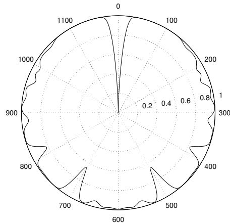
Figure 7. Spectral pitch-class distances of all pitch-class intervals. The size of the interval increases around the circle and is labelled in cents (one hundredths of a 12-TET semitone). The spectral pitch-class distance is 0 at the centre of the circle and 1 at the perimeter. The roll-off and smoothing parameters are as optimized to the data. The symmetry about the vertical axis results from the use of spectral pitch classes rather than pitches.
