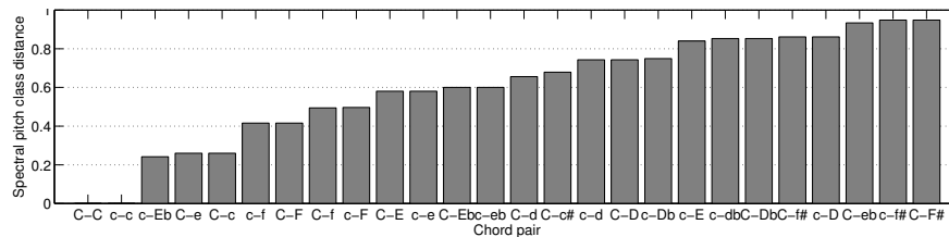
Figure 8. Spectral pitch-class distances, in order, of all chord pairs. The roll-off and smoothing parameters are as optimized to the data.
