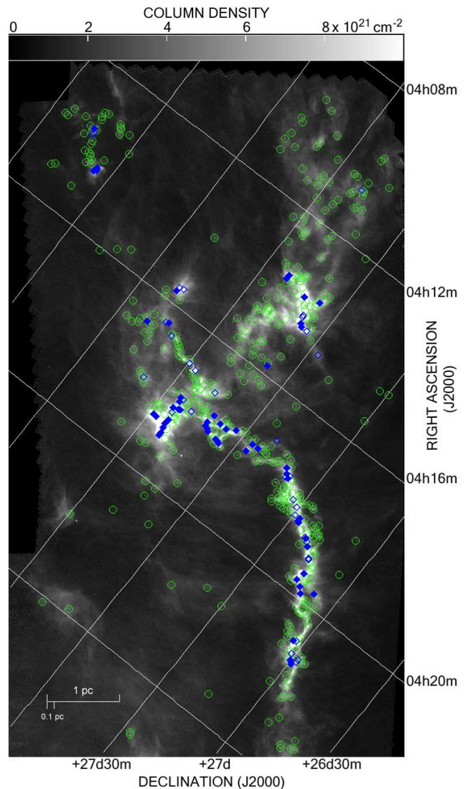
Figure 1. Column density map of the region studied. The spatial resolution is approximately 18.2'' and the column density units are hydrogen molecules per \text{cm}^2 . The overplotted symbols represent the locations of detected cores (green circles = unbound starless, filled blue diamonds = prestellar, open blue diamonds = candidate prestellar). The peak column density is 5.5 \times 10^{22} \text{ cm}^{-2} , although the display scale is truncated at 1.0 \times 10^{22} \text{ cm}^{-2} to improve the visibility of faint features.
