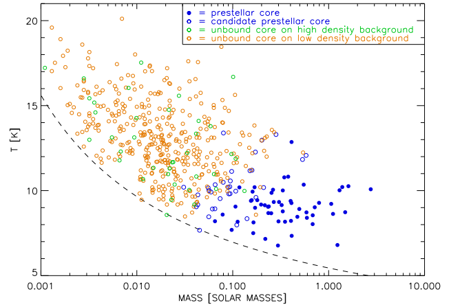
Figure 4. Estimated mean dust temperature plotted as a function of estimated core mass. Bound (prestellar) cores and prestellar core candidates are plotted as filled and open blue circles, respectively. Unbound cores are represented by open circles and are divided into those seen against high column density backgrounds characterised by A_V > 7 mag (green symbols), and more diffuse backgrounds (gold symbols). The dashed line represents the detection limit, i.e., the lowest detectable mass for a given core temperature.
