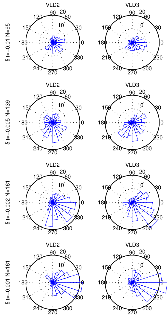
FIG. 6. Polar plots of histograms of VLD2 (left panels) and VLD3 (right panels) temporal analytic phase difference \Delta\phi just before an ELM in the flat-top of JET plasma 83771. The same data and analysis are used as in Figure 5 except that now Hilbert transform time window (b) is used to determine the VLD temporal analytic phases and it stops at t_{ELM2} , the time of the second ELM. Phase differences can then only be determined for times \delta t > \delta t_E = 1\text{ms} before t_{ELM2} . From bottom to top \delta t = [1, 2, 5, 10] ms.
