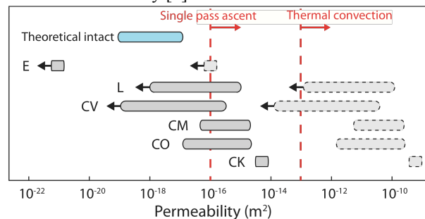
Fig. 1. Summary of laboratory (dark gray; [10, 11]) and theoretical (blue; [9]) permeabilities for chondrites. Light gray values with dashed outlines represent laboratory permeabilities augmented by 10^5 to account for the effects of fractures and scale (see text). Black arrows indicate meteorite groups that have at least one sample with permeability below the detection threshold of the experimental setup.
