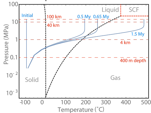
Fig. 2. Evolution of the interior temperatures of a 200 km diameter planetesimal accreted 1.3 My after CAIs overlaid on the water phase diagram. Blue curves indicate the temperature profiles at the specified times. Although we assume only conductive cooling in a body with uniform thermal diffusivity, pore fluid convection may occur in the near-surface zone of large temperature gradients given sufficiently high permeability [8].
