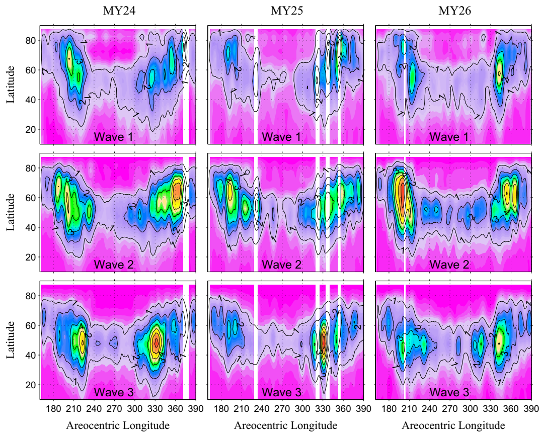
Fig. 9. Seasonal evolution of the RMS eddy T field (in K) in the northern hemisphere for MY24 (left column), MY25 (middle column) and MY26 (right column), arranged by contribution from zonal wavenumbers 1, 2 and 3, in the top, middle, and bottom rows, respectively. As in Fig. 7, the eddy field is on the 0.83 sigma surface and filtered as in Fig. 1. Contours are drawn every 1 K, with the outer (lowest) contour at 1 K and shaded for emphasis. The periods during which there are no TES retrievals available are indicated here by an absence of shading.
