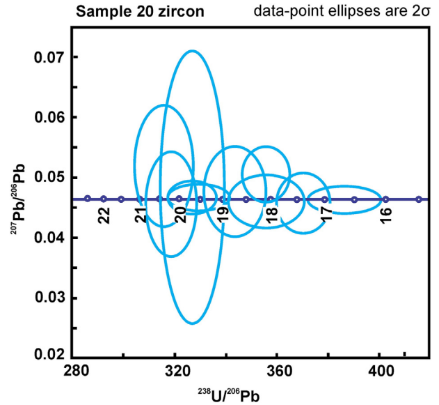
Fig. 9. Tera–Wasserburg zircon U–Pb data plot for sample 20 (Ludwig, 2003) with 2σ error ellipses.
