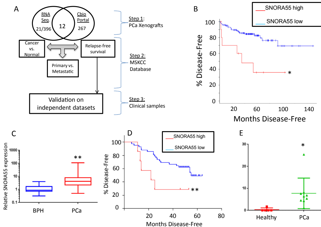
Figure 1 – A, Analytical strategy employed for this study. 21 out of 396 differentially expressed snoRNAs (Met. vs. Non-met. xenografts) were searched in the MSKCC database containing 267 snoRNAs. 12/21 genes were also represented in this platform and were chosen for further analyses. The gene(s) associated with PCa prognosis were validated in an independent clinical dataset. B, Relapse-free survival according to SNORA55 expression in primary tumor at diagnosis, (MSKCC database, dichotomization based on Z score, as described in “Methods”) * p < 0.05 (log rank test, Bonferroni correction). C, SNORA55 expression measured by qPCR in 9 BPH and 43 primary PCa samples. ** p < 0.01 (unpaired T test). D, Relapse-free survival according to SNORA55 expression in primary tumor at diagnosis (qPCR on 43 samples). ** p < 0.01 (log rank test). E, Expression of SNORA55 in serum samples from PCa patients and healthy controls. * p < 0.05 (unpaired, two-sided T test).
