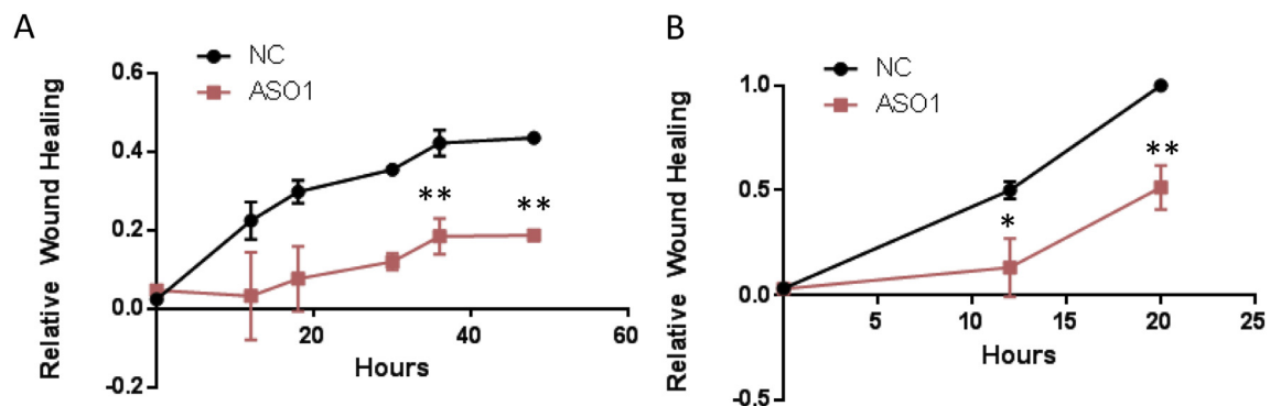
Figure 4 – LNCaP (A) and Du145 (B) cell migration in cells exposed to control or ASO1 (250 nM). * p < 0.05 ; ** p < 0.01 (2 way ANOVA and Sidak post-test).
