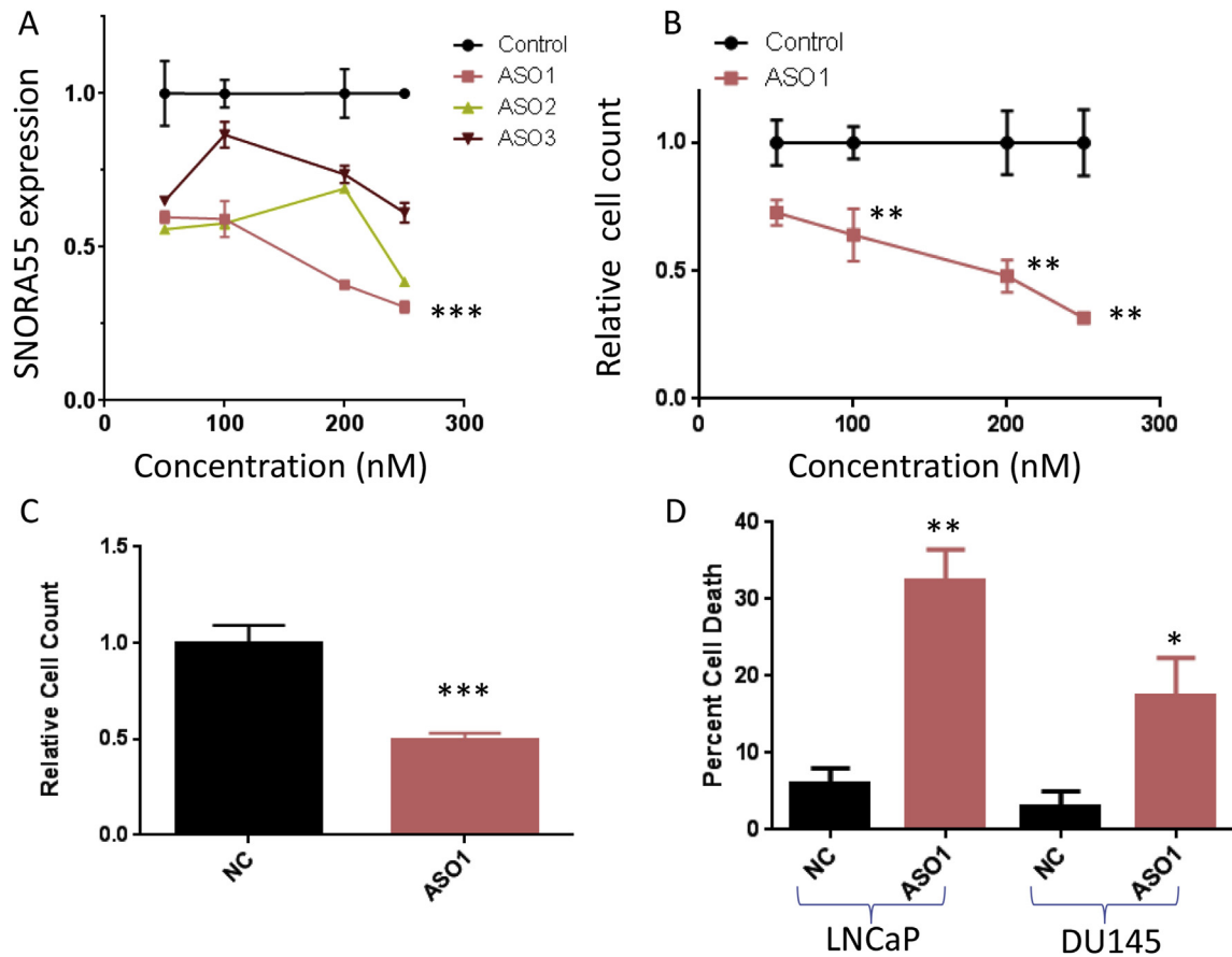
Figure 3 – A, SNORA55 expression in LNCaP cells exposed to different ASO concentrations (48 h). *** p < 0.001 vs. control (1 way ANOVA and Tukey multiple comparison post-test, highest concentration of each treatment). B, Relative LNCaP cell count after treatment with different ASO concentrations (48 h). ** p < 0.01 (2 way ANOVA and Sidak post-test). C, Relative DU145 cell count after treatment with ASOs (250 nM, 48 h). *** p < 0.001 (unpaired T test). D, Percentage of cell death in LNCaP and DU145 cells exposed to NC or ASO1 (250 nM, 48 h). * p < 0.05 ; ** p < 0.01 (unpaired T test).
