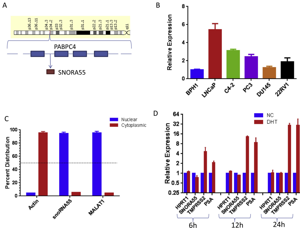
Figure 2 – A, Chromosomal localization of SNORA55 (data from Gene Cards). B, SNORA55 expression in prostate cell lines. C, Subcellular localization of SNORA55 in LNCaP cells (MALAT1 is a nuclear non-coding RNA, actin mRNA is prevalently cytoplasmic). D, Effects of DHT treatment on SNORA55 expression (LNCaP cells). HPRT1 is an AR-independent gene (negative control), PSA and TMPRSS2 are AR-dependent genes (positive controls). The experiment was performed as previously described (Parolia et al., 2015).
