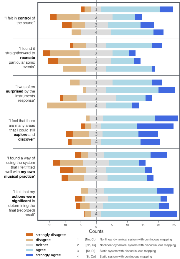
Figure 3. Participant agreement with six different statements in Section 4.2 as they apply to the four different musical interfaces described in Section 4.1.
