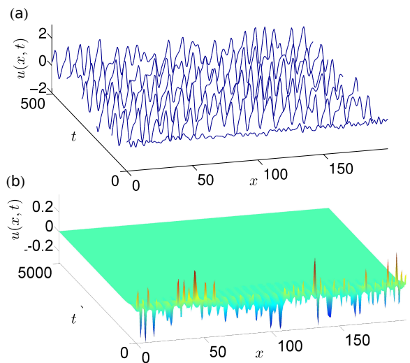
FIG. 4: (Color online) Computations of the KS equation \delta = 0 for the extended domain L = 200 (see also “movieDelta0.avi” in Supplemental Material [24]). (a) Uncontrolled solution. (b) The zero solution is stabilized by using m = 63 controls.
