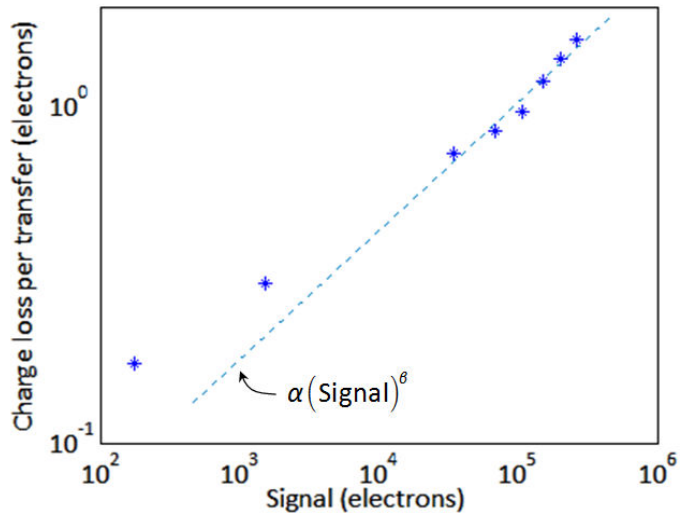
Figure 6. Charge loss per transfer for increasing signal levels. Experimental data from Extended Pixel Edge Response (EPER) data is shown by the points, with the functional form of a simple power law shown by the dashed line (i.e. without the additional \gamma parameter). The power law is insufficient to accurately map the functional form of the data and the \gamma parameter is required.
