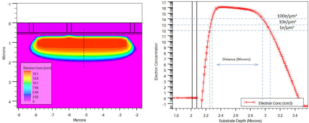
Figure 4. Left: Cut through 3D Silvano simulation of charge storage in a CCD [23]. Right: One-dimensional profile through the left-hand charge storage simulation, showing the steep increase in density (noting the logarithmic electron density scale) [23].
