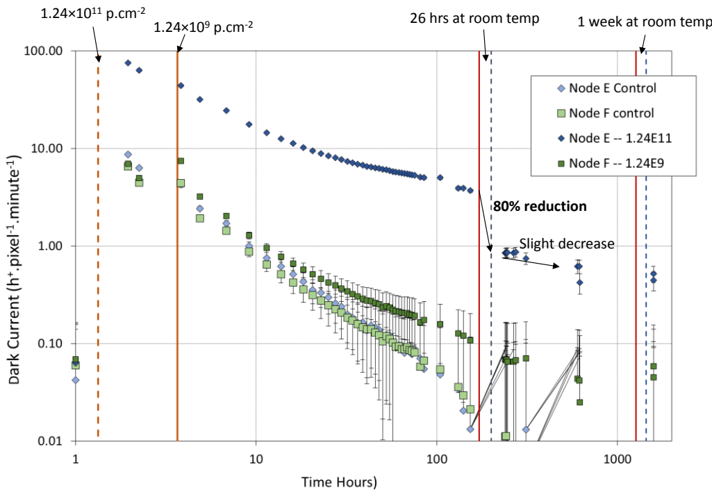
Figure 8. Dark current as a function of time in the two irradiated regions and their respective control regions
