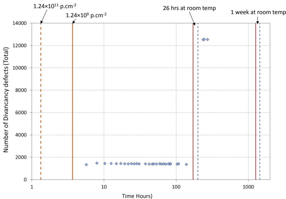
Figure 13. Number of divacancy defects recorded after the irradiation as a function of time
