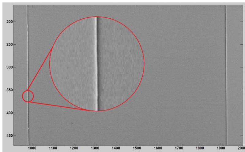
Figure 11. Image taken using a flat field exposure of 20,000 holes, cropped to show the area irradiated with a 10 MeV equivalent fluence of 1.24 \times 10^{11} protons.cm -2 and the charge redistribution which occurs on the boundaries of the irradiation
