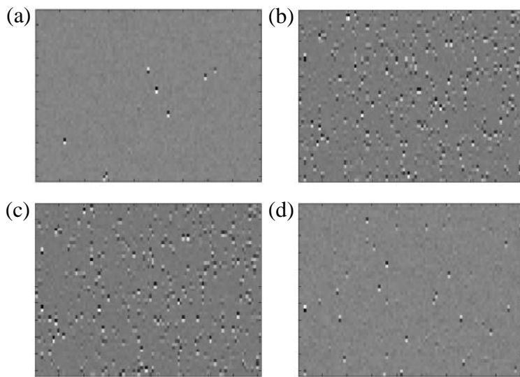
Figure 15. Image showing the results of trap pumping in a section of the device pre-irradiation (a), 6 minutes after the irradiation was complete (b), 18 minutes after the irradiation was complete (c) and a difference image (d) showing the change over a period of 12 minutes
