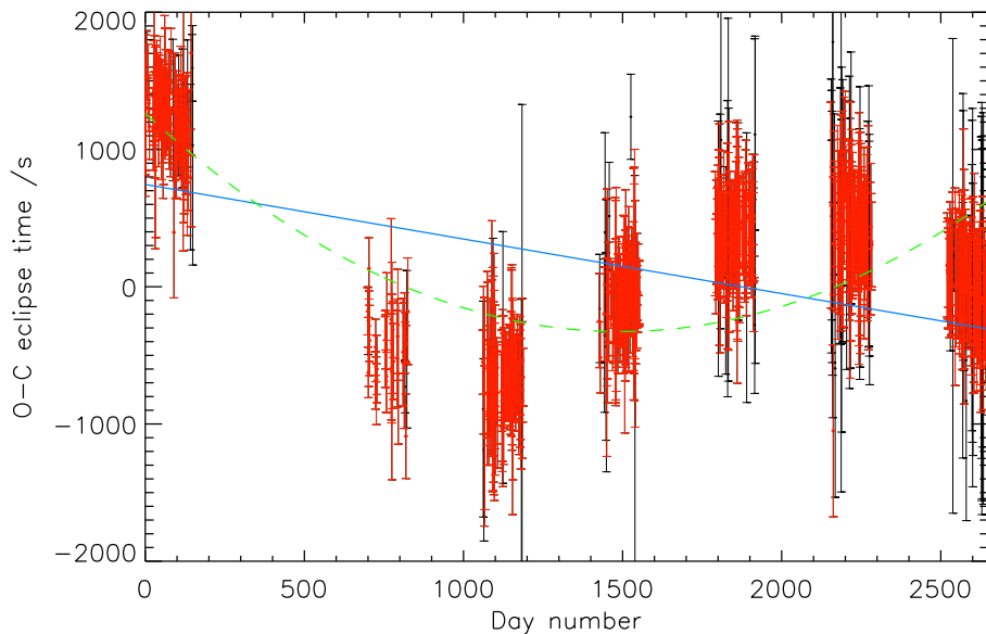
Figure 2. O - C diagram for a SuperWASP eclipsing binary candidate exhibiting sinusoidal variation. Linear (solid line) and quadratic (dashed line) best fits are overplotted; neither matches the period variation well.
