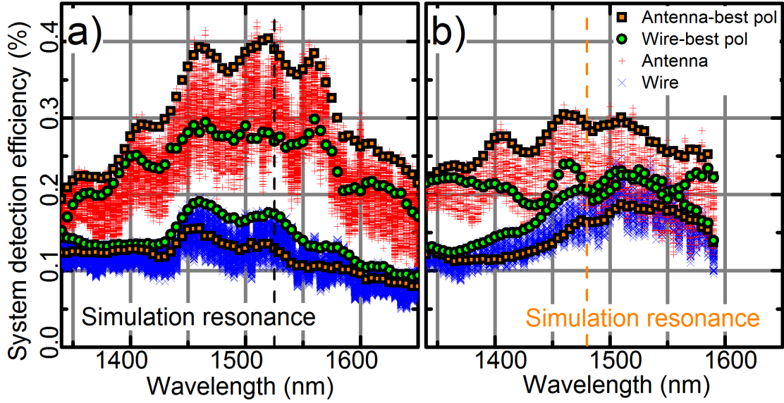
Figure 2: By sweeping the wavelength from 1340nm to 1650nm in 5nm steps and normalizing out the photon flux using a separate power measurement it is possible to observe the range of efficiencies at each wavelength across the full polarization space. By using an electronic polarization controller these polarizations are made repeatable, which allows post-measurement selection of efficiencies at a given polarization across multiple separate measurements. In both figures, red pluses represent data obtained when illuminating an antenna, while blue crosses represent data obtained illuminating a bare wire. In figure 2a the polarizations at which the \lambda_{res} = 1525 nm nanoantenna and wire respond best are selected. Figure 2b shows the response for the \lambda_{res} = 1480 nm nanoantenna. The peak value data for these figures was averaged over the four adjacent points to smooth out the interference. There is clear agreement between the peak efficiency value and the simulation's suggested resonance (shown as a dashed line, comparable with figure 1d). Figure 2a sampled 256 polarizations per wavelength while figure 2b sampled 64: separate testing showed no improvement using 256 points over 64, and it was quicker to measure fewer polarizations.
