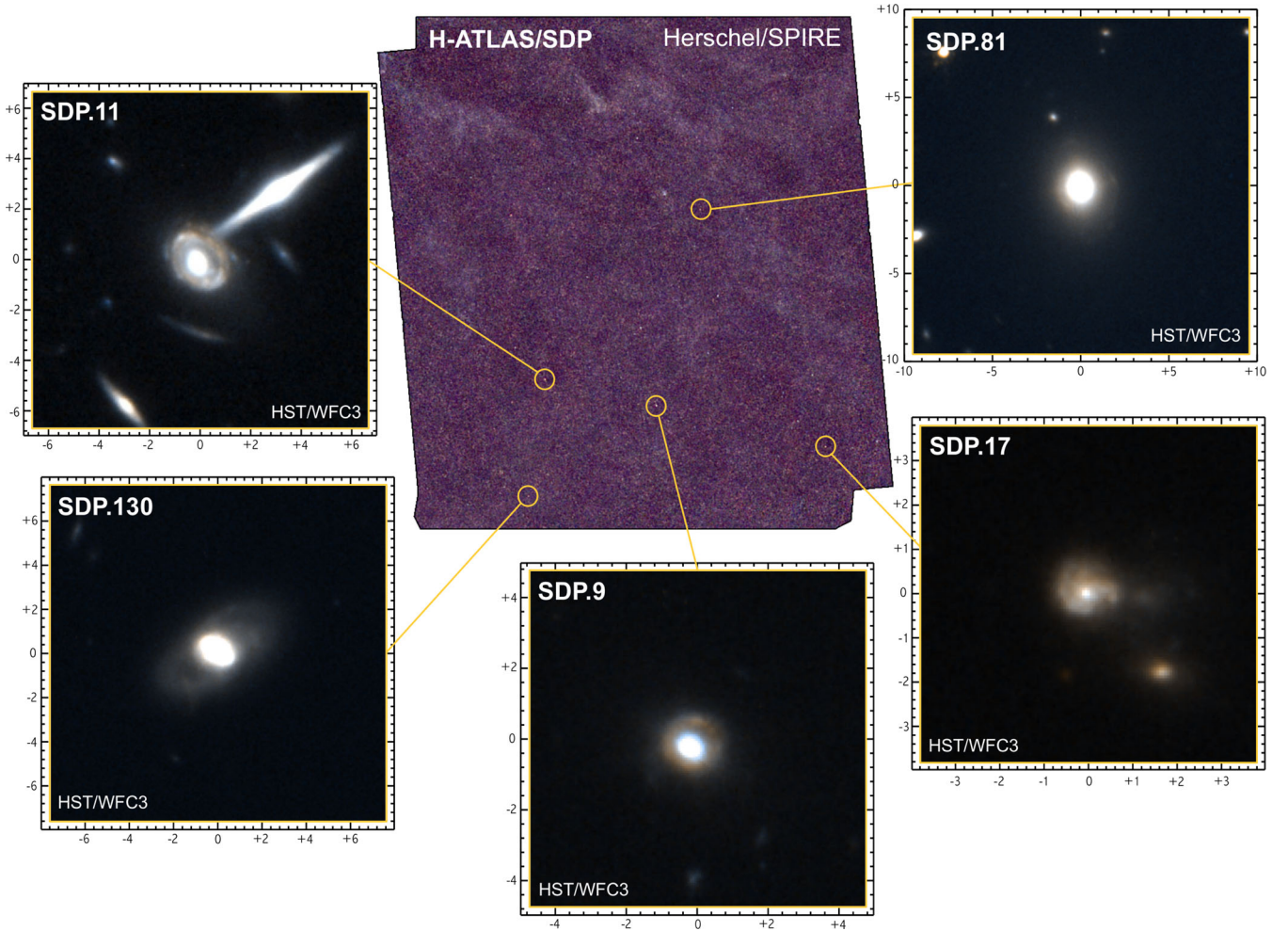
Figure 1. Two-colour postage stamp HST /WFC3 images of the first five confirmed gravitational lensing systems discovered by H-ATLAS (blue for F110W and red for F160W). The position of the five sources in the Herschel /SPIRE map of the H-ATLAS SDP field is indicated by the yellow circles. The scale of the postage stamps is given in arcseconds.
