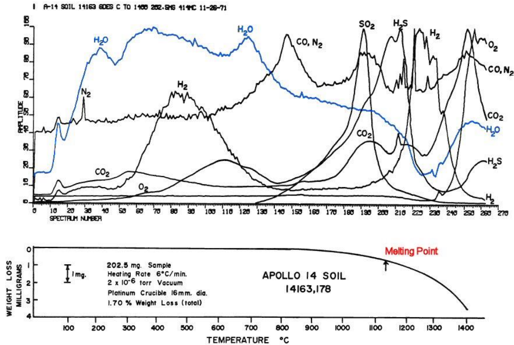
Figure 2. Evolved gas release from Apollo 14 lunar soil 14163 [7]. Volatiles released during heating lunar soil 14163 at 6°C/min from room temperature to 1400°C. Gas releases are normalized to 100% at the temperatures of greatest abundance.
