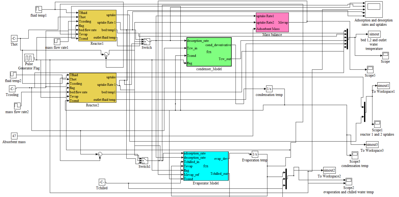
Figure 2: Arrangement of chiller component in Simulink simulation environment
