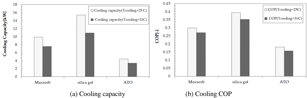
Fig. 8. Effect of cooling water temperature on the chiller cooling capacity and COP
