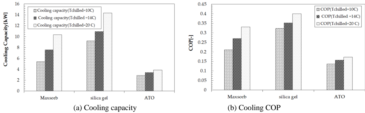
Fig. 7. Effect of chilled water temperature on the chiller cooling capacity and COP
