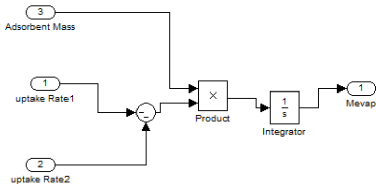
Figure 3a: Integration Block in Simulink
