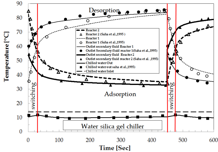
Figure 4: Validation of water/silica gel chiller
