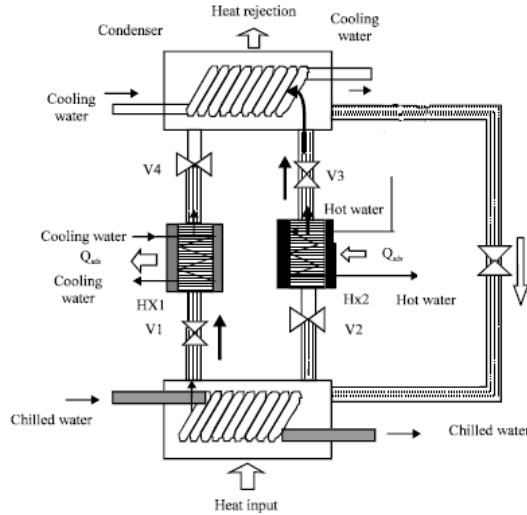
Figure1: Schematic of Two bed adsorption chiller
