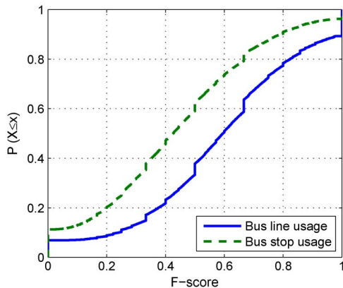
Fig. 5. CDF of the F-score values among all riders for bus line and bus stop usage predictability. Each rider is associated with the highest F-score that has been achieved among all predictors.
