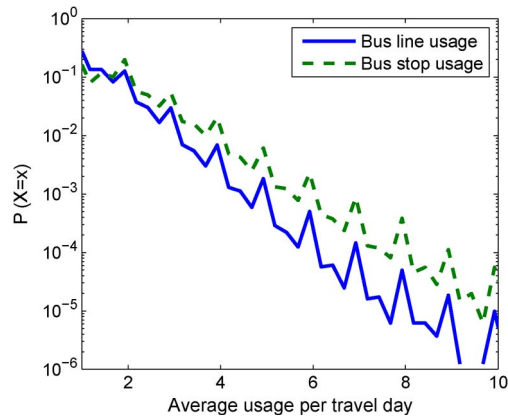
Fig. 3. Probability distribution of a rider's average daily usage, differentiating between stops and lines used. The distribution of bus stop usage is more skewed than bus line usage.
