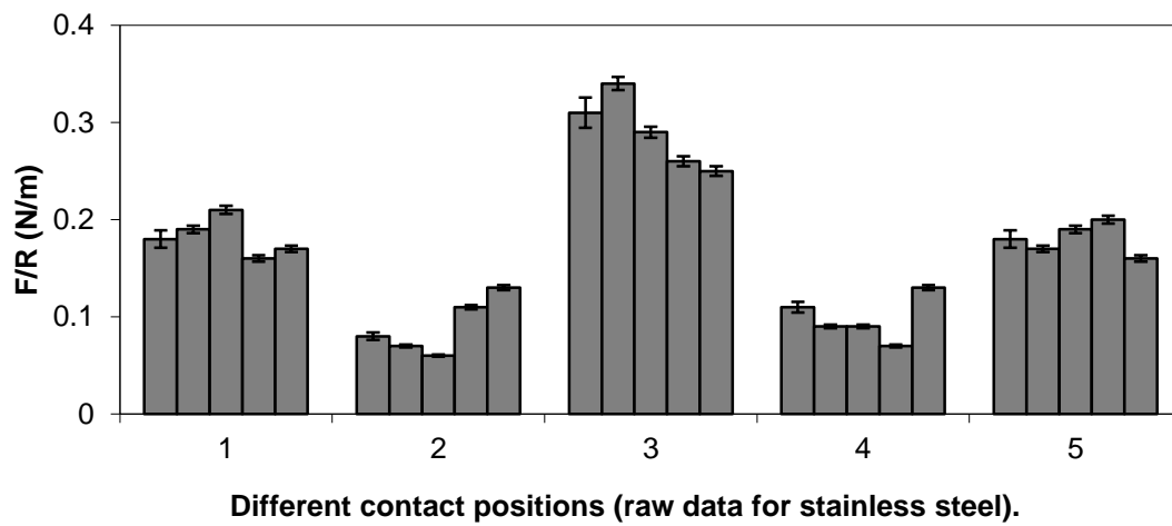
Figure 3. Interaction between stainless steel microparticles and caramel, measured using the AFM. Data shows local variation of 5 points at each of the 5 regions on the caramel deposit; error bar shows the equipment error per measurement.
