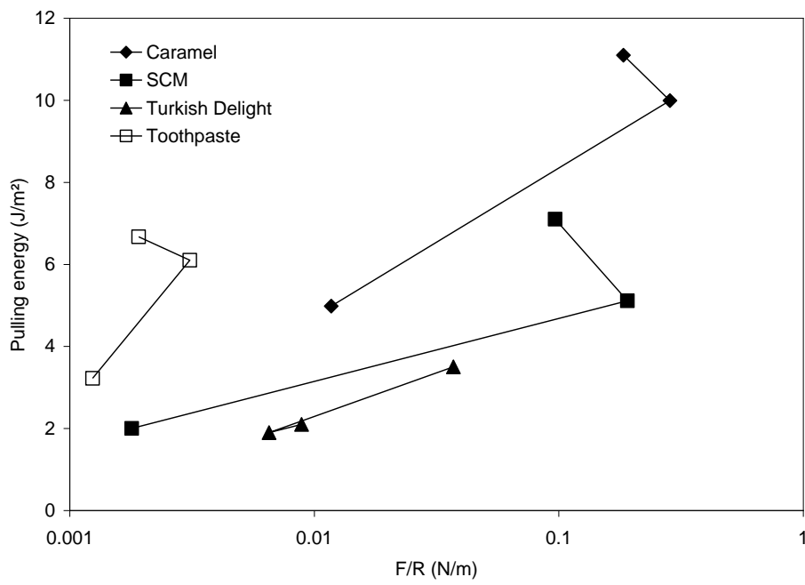
Figure 8. Comparison of data from micromanipulation and AFM, plotted for each deposit type.
