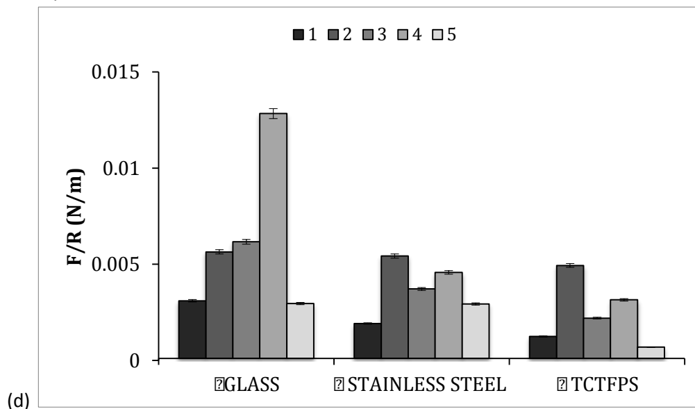
Figure 4. AFM force measurements. Glass, stainless steel and TCTFPS microparticles were immersed in deposits and then retracted. Deposits were spread 50 - 60 \mu m thick on a glass slide. Data shows results from five different contact positions (1-5) on the deposits. The approach speed for all experiments was 3 \mu m/s, followed by a 5 second pause on deposit and 0.25 \mu m/s retract. Deposits are (a) caramel, (b) SCM, (c) Turkish delight, (d) toothpaste;
